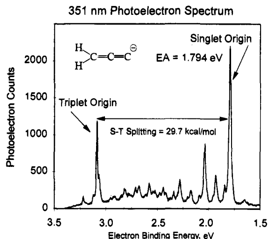
Figure 4. The photoelectron spectrum of the propadienylidene anion ( \text{CH}_2=\text{C}=\dot{\text{C}}^- ) exhibits transitions to both the singlet ground state and triplet excited state of the propadienylidene diradical ( \text{CH}_2=\text{C}=\dot{\text{C}} ).
