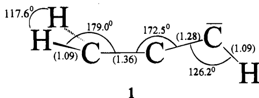
Figure 5. Optimized geometry for the C 3 H 3 - anion at the MP2(FU)/6-311+G** level of theory using Gaussian 92 (ref 40). Bond lengths (in parentheses) are in Angstroms.
